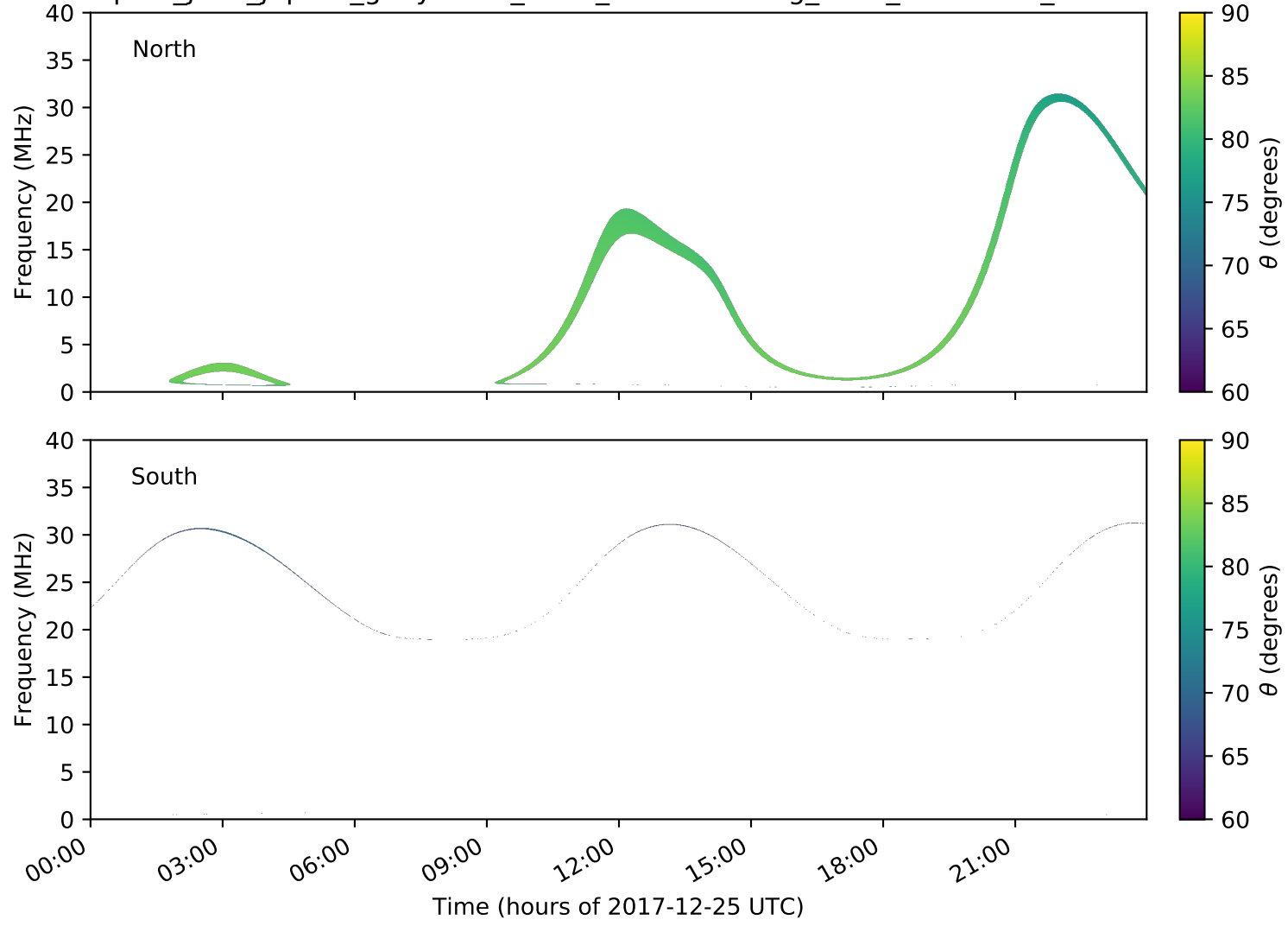
expres_juno_jupiter_ganymede_isaac_lossc-wid1deg_3kev_20171225_v01.cdf
