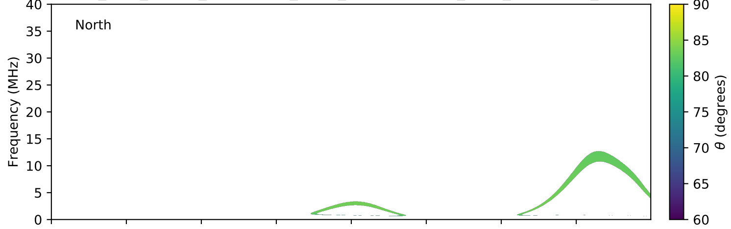
expres_juno_jupiter_ganymede_isaac_lossc-wid1deg_3kev_20171218_v01.cdf
