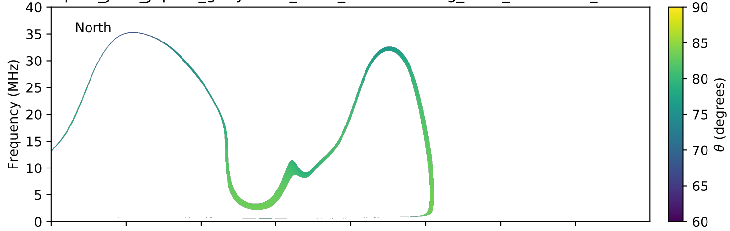
expres_juno_jupiter_ganymede_isaac_lossc-wid1deg_3kev_20171213_v01.cdf
