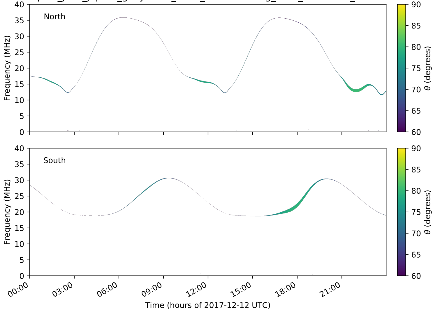
expres_juno_jupiter_ganymede_isaac_lossc-wid1deg_3kev_20171212_v01.cdf
