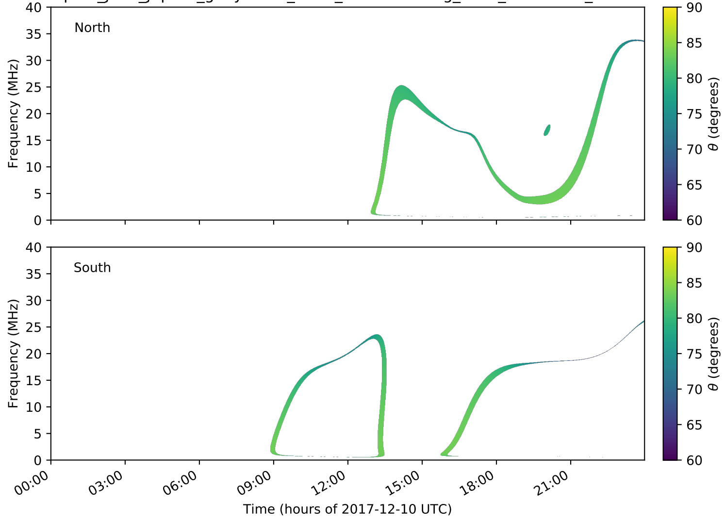
expres_juno_jupiter_ganymede_isaac_lossc-wid1deg_3kev_20171210_v01.cdf
