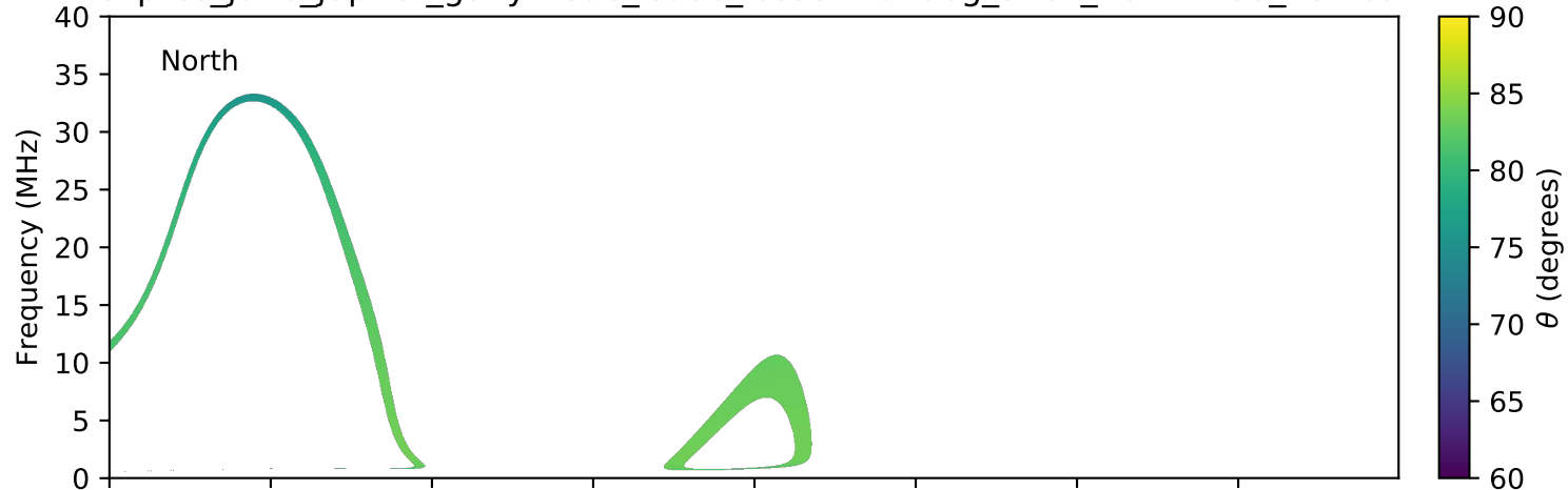
expres_juno_jupiter_ganymede_isaac_lossc-wid1deg_3kev_20171206_v01.cdf
