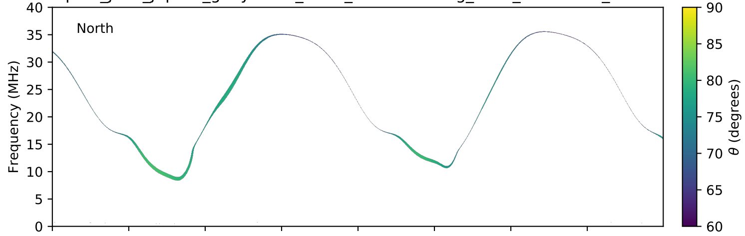
expres_juno_jupiter_ganymede_isaac_lossc-wid1deg_3kev_20171204_v01.cdf
