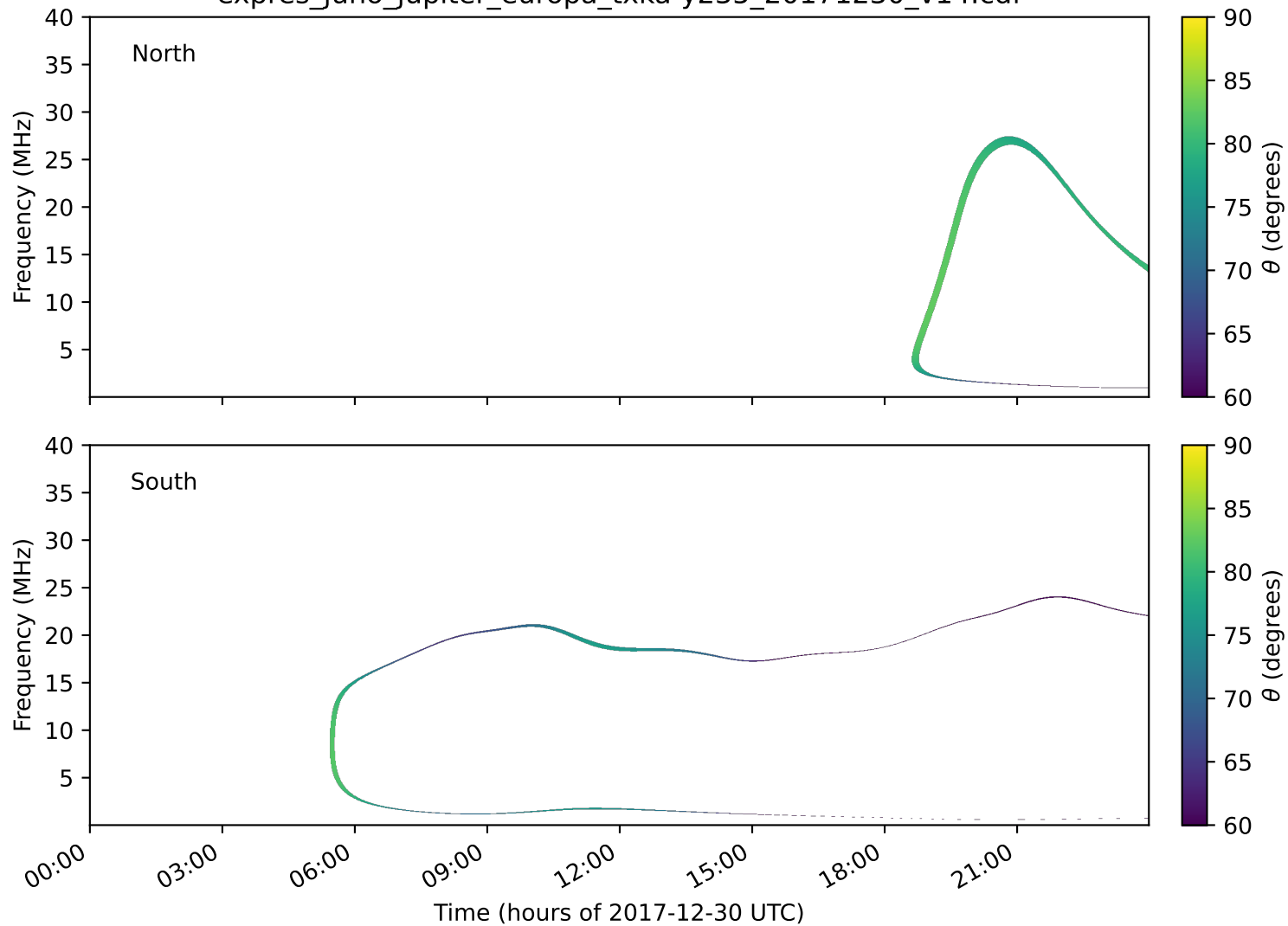
expres_juno_jupiter_europa_txka-y235_20171230_v14.cdf
