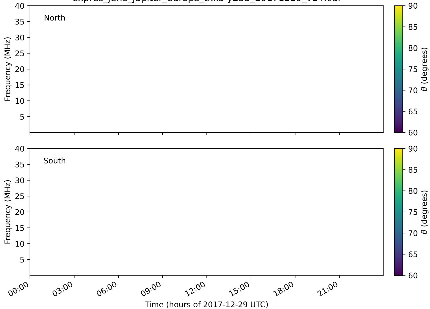
expres_juno_jupiter_europa_txka-y235_20171229_v14.cdf
