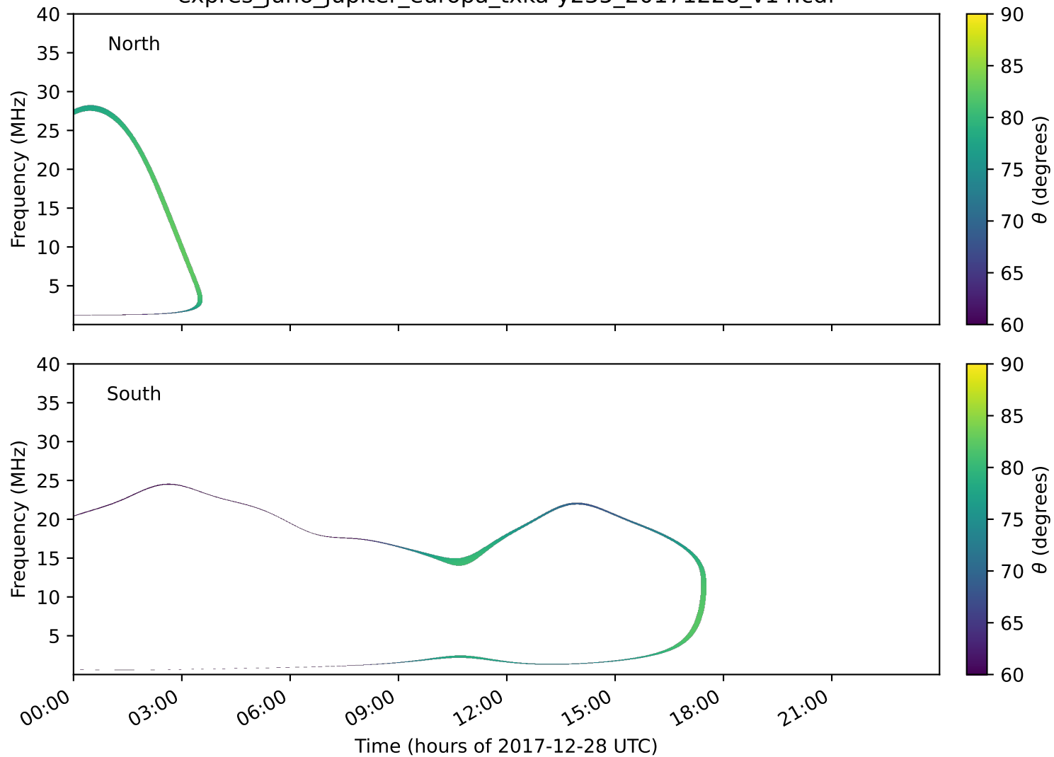
expres_juno_jupiter_europa_txka-y235_20171228_v14.cdf
