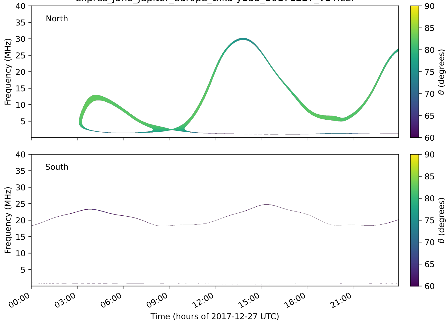
expres_juno_jupiter_europa_txka-y235_20171227_v14.cdf
