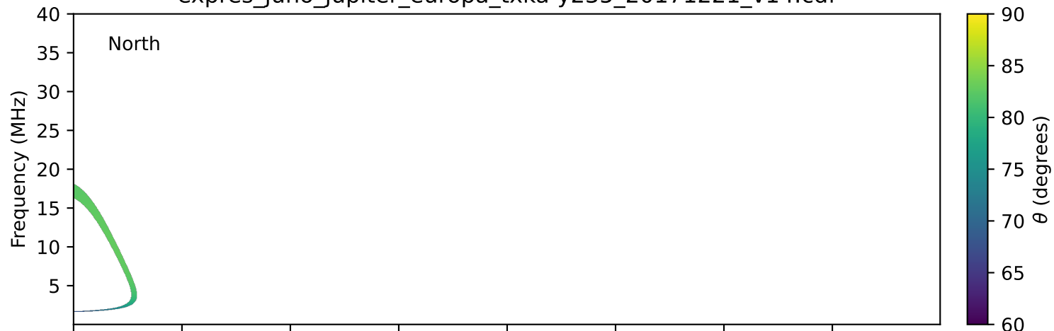
expres_juno_jupiter_europa_txka-y235_20171221_v14.cdf
