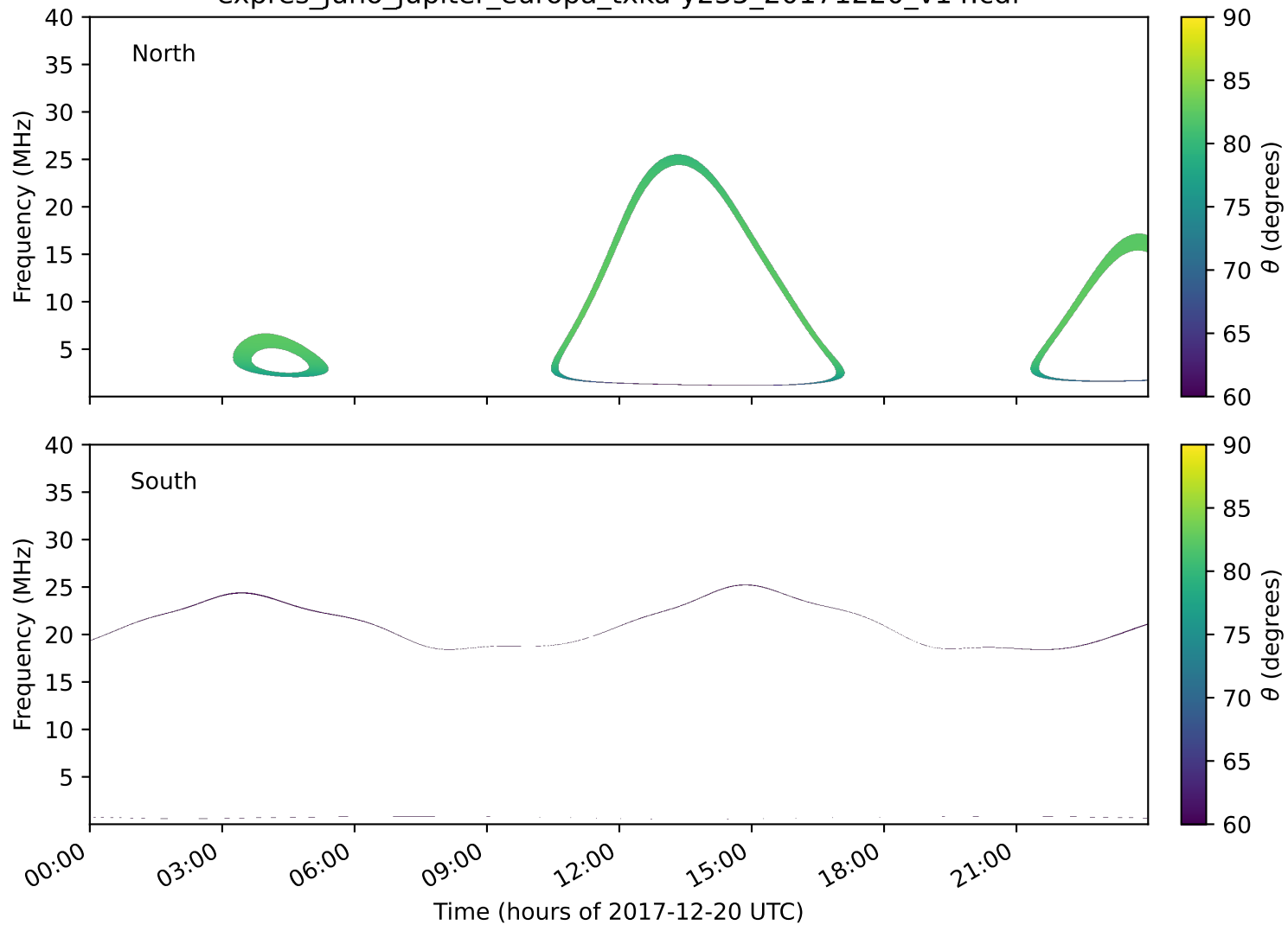
expres_juno_jupiter_europa_txka-y235_20171220_v14.cdf
