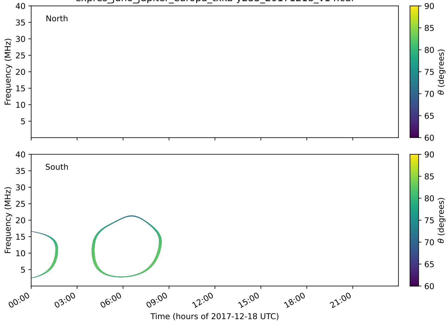
expres_juno_jupiter_europa_txka-y235_20171218_v14.cdf
