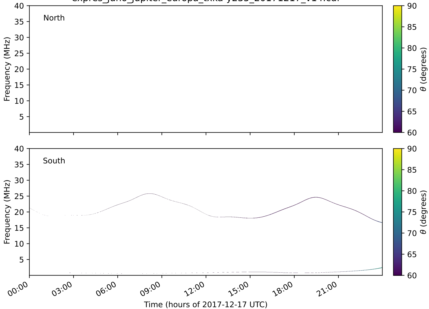
expres_juno_jupiter_europa_txka-y235_20171217_v14.cdf
