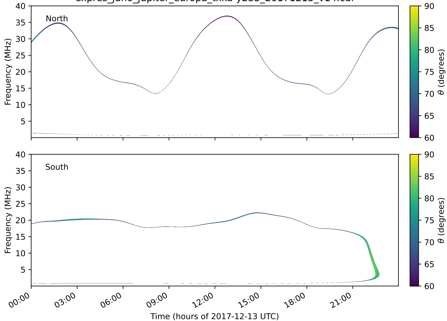
expres_juno_jupiter_europa_txka-y235_20171213_v14.cdf
