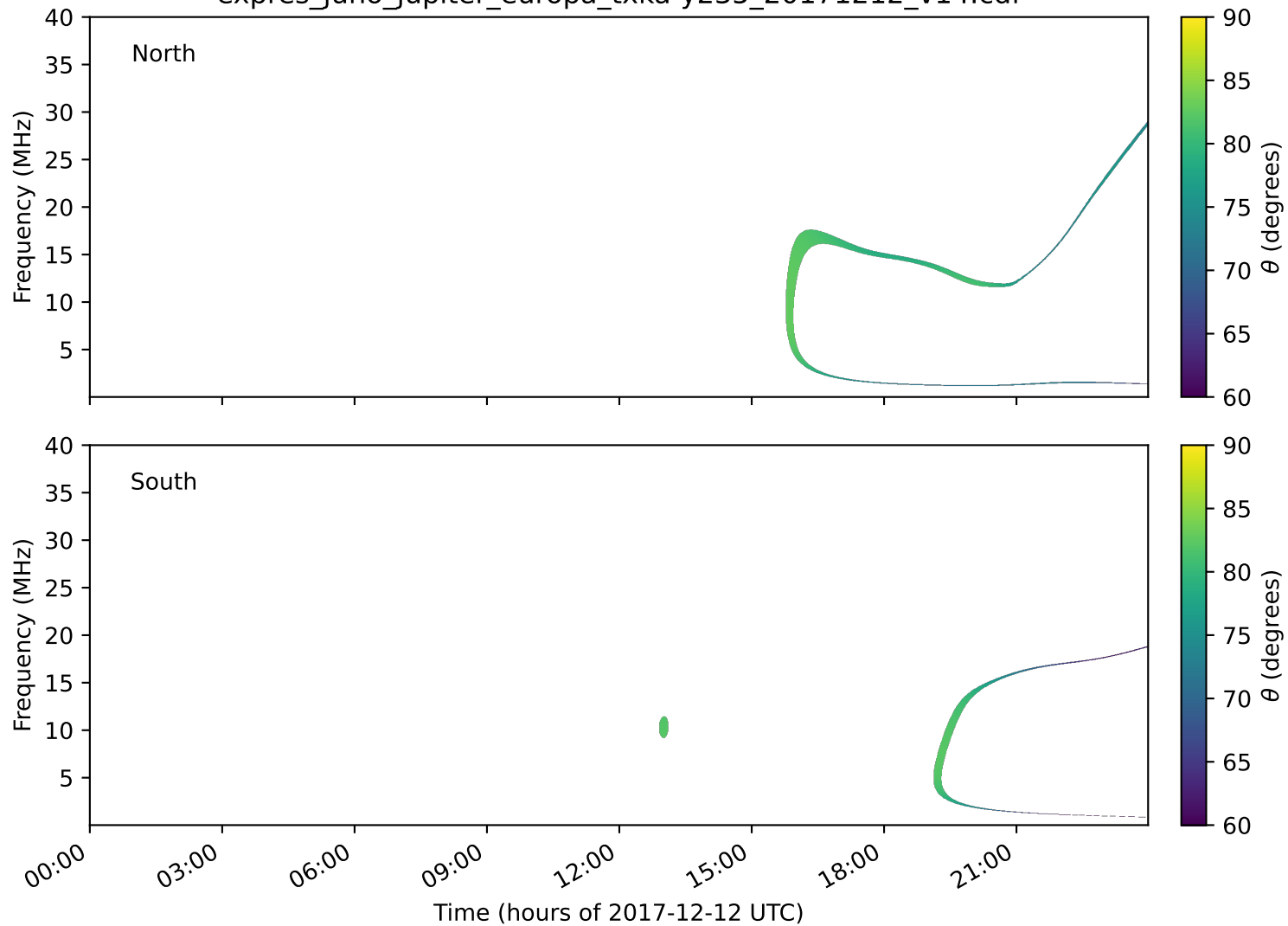
expres_juno_jupiter_europa_txka-y235_20171212_v14.cdf
