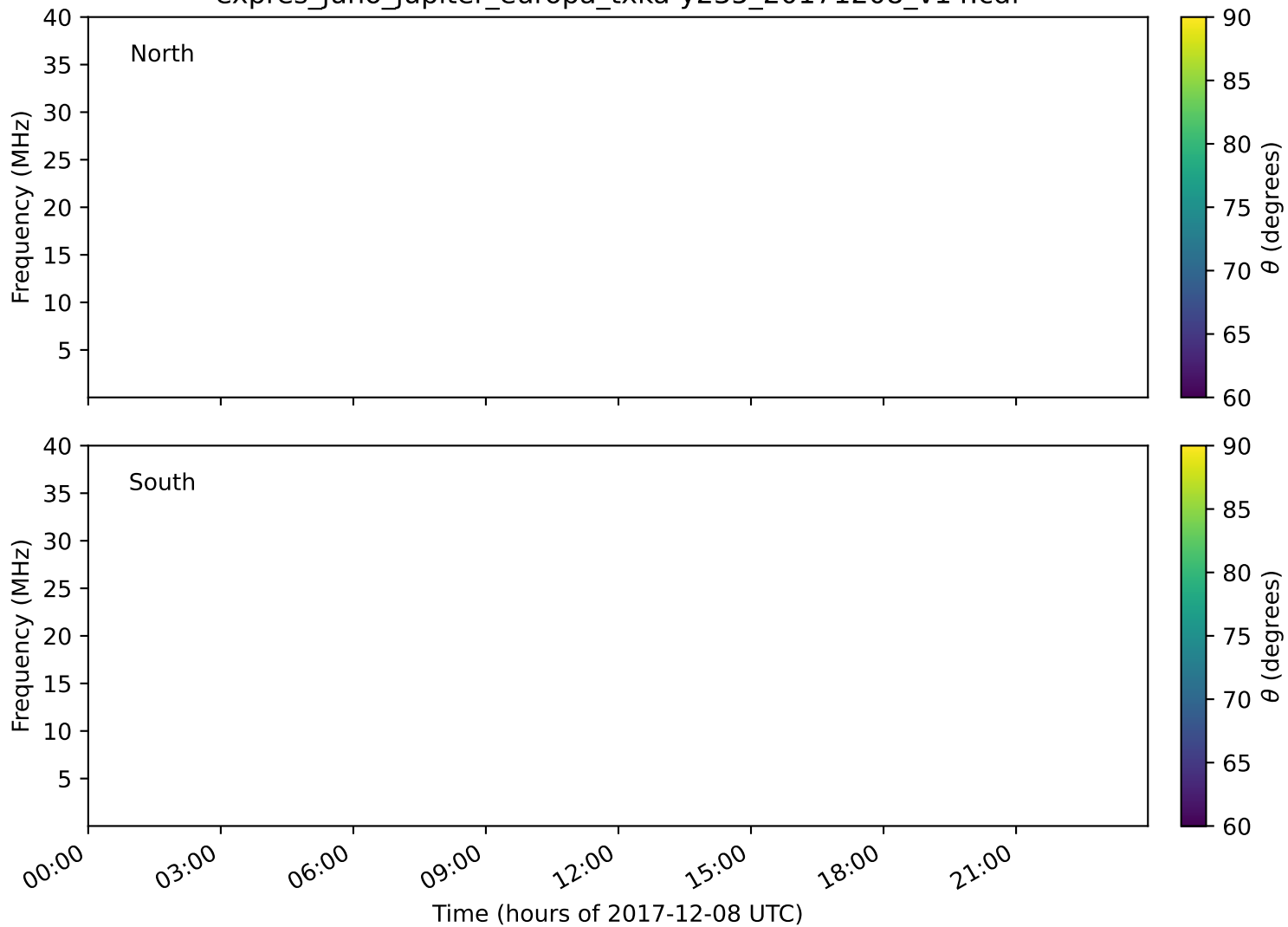
expres_juno_jupiter_europa_txka-y235_20171208_v14.cdf
