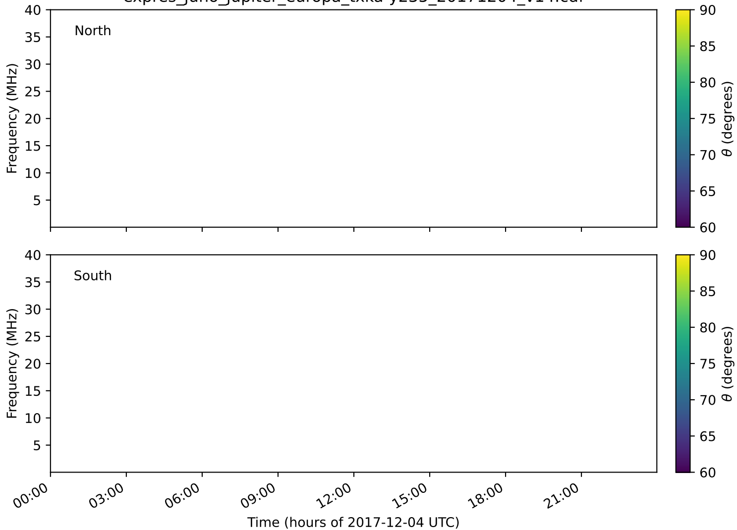
expres_juno_jupiter_europa_txka-y235_20171204_v14.cdf
