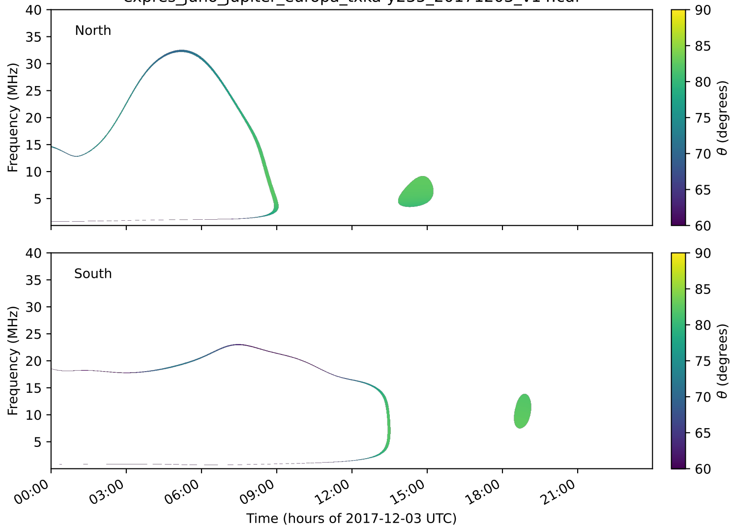
expres_juno_jupiter_europa_txka-y235_20171203_v14.cdf
