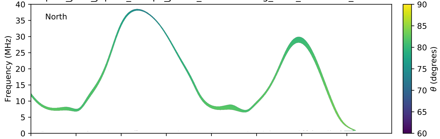
expres_juno_jupiter_europa_jrm09_lossc-wid1deg_3kev_20171231_v01.cdf
