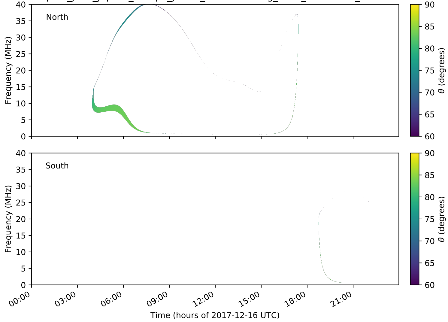
expres_juno_jupiter_europa_jrm09_lossc-wid1deg_3kev_20171216_v01.cdf
