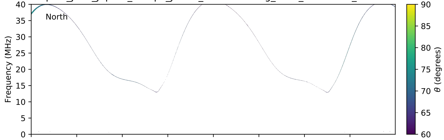
expres_juno_jupiter_europa_jrm09_lossc-wid1deg_3kev_20171213_v01.cdf
