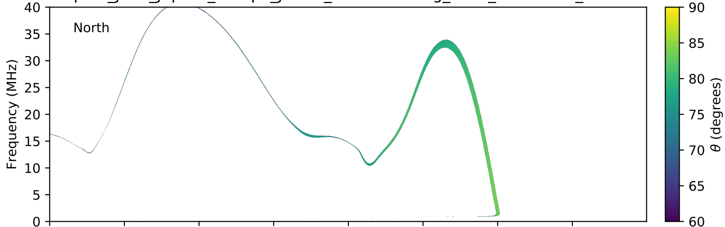
expres_juno_jupiter_europa_jrm09_lossc-wid1deg_3kev_20171210_v01.cdf
