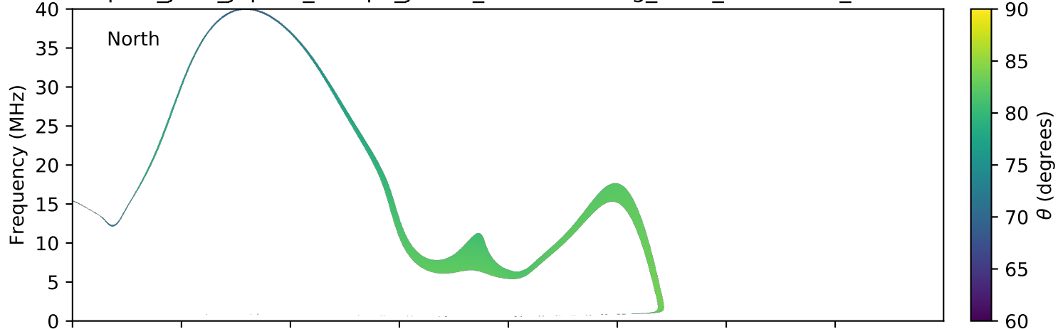
expres_juno_jupiter_europa_jrm09_lossc-wid1deg_3kev_20171203_v01.cdf
