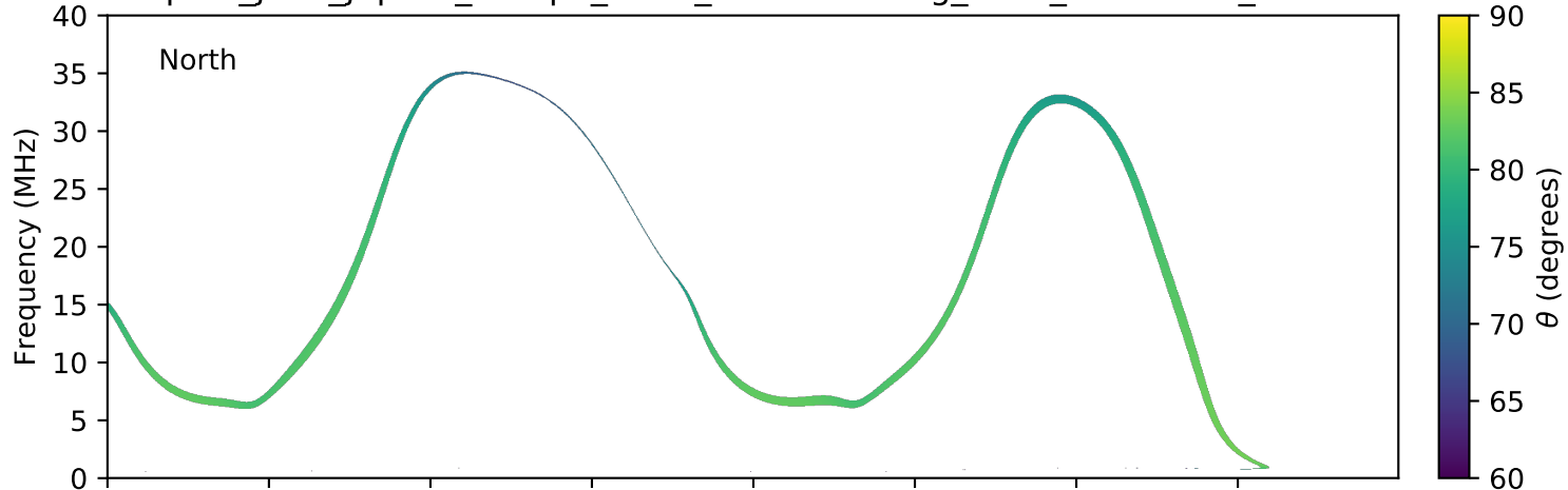
expres_juno_jupiter_europa_isaac_lossc-wid1deg_3kev_20171231_v01.cdf
