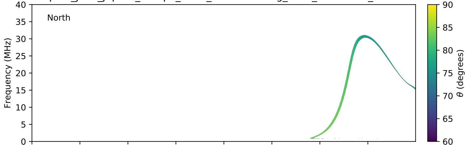
expres_juno_jupiter_europa_isaac_lossc-wid1deg_3kev_20171230_v01.cdf
