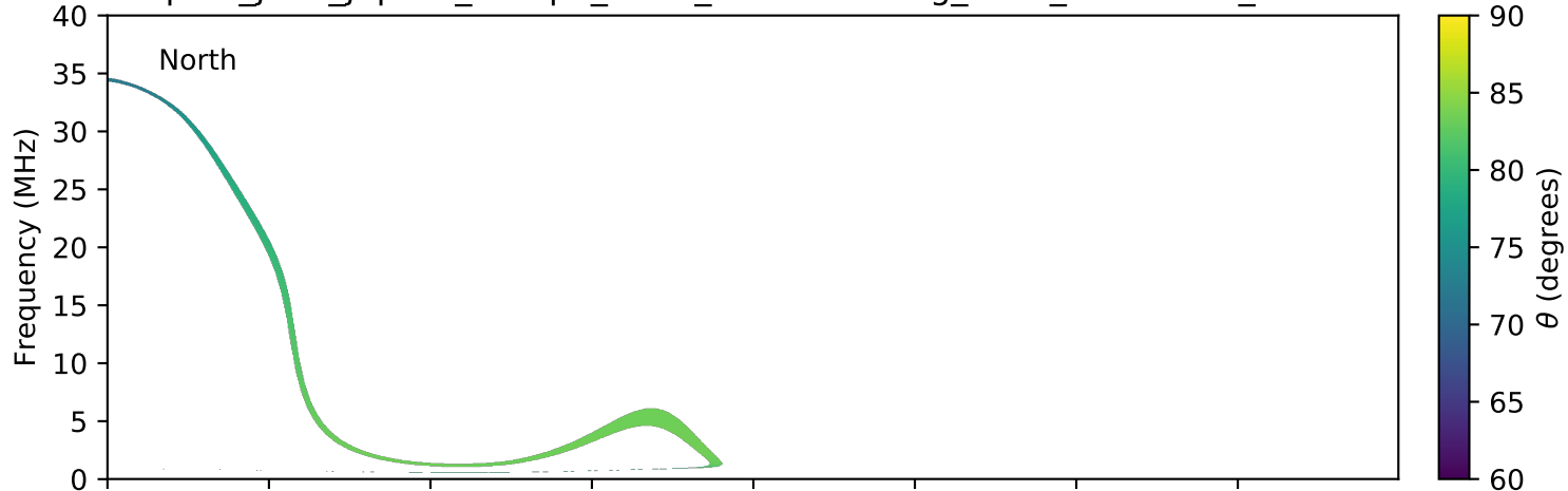
expres_juno_jupiter_europa_isaac_lossc-wid1deg_3kev_20171228_v01.cdf
