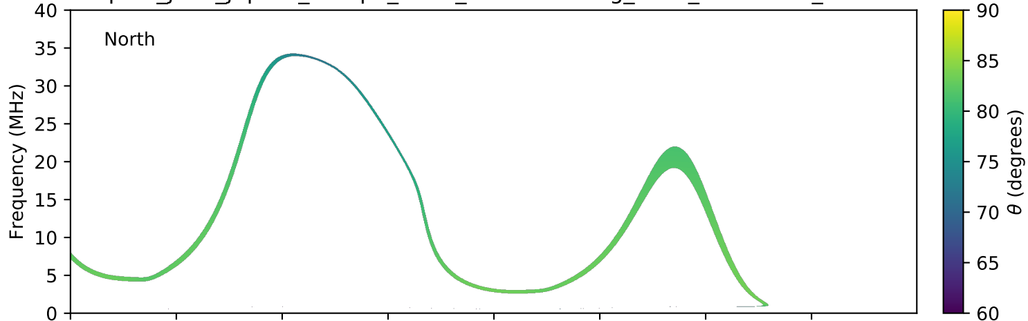
expres_juno_jupiter_europa_isaac_lossc-wid1deg_3kev_20171224_v01.cdf
