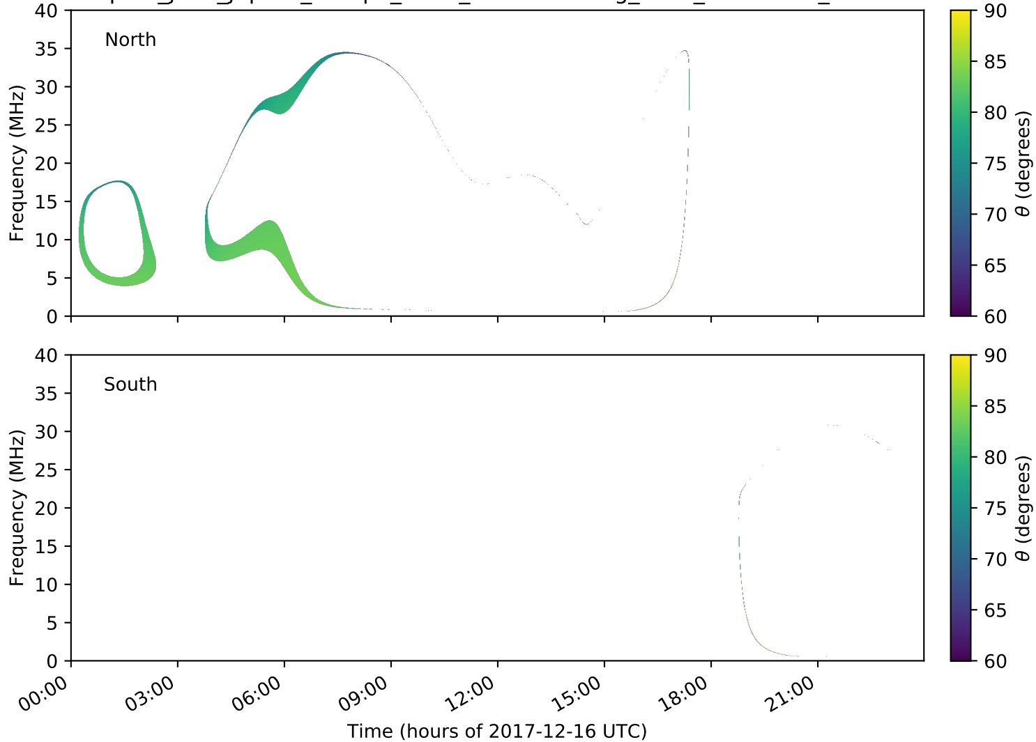
expres_juno_jupiter_europa_isaac_lossc-wid1deg_3kev_20171216_v01.cdf
