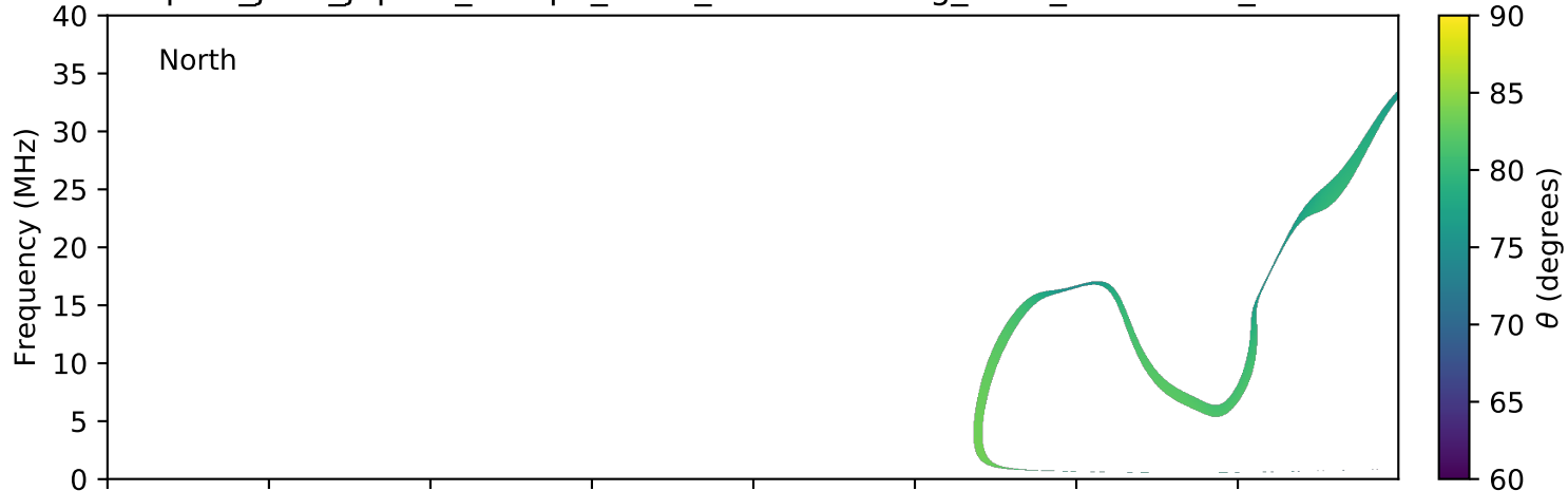
expres_juno_jupiter_europa_isaac_lossc-wid1deg_3kev_20171212_v01.cdf
