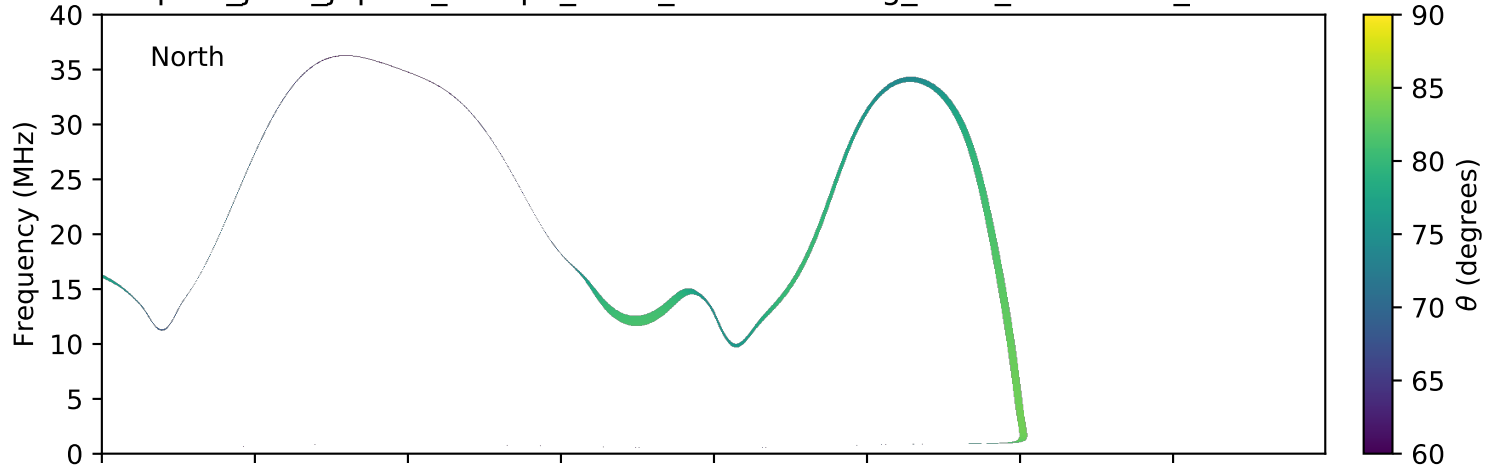
expres_juno_jupiter_europa_isaac_lossc-wid1deg_3kev_20171210_v01.cdf
