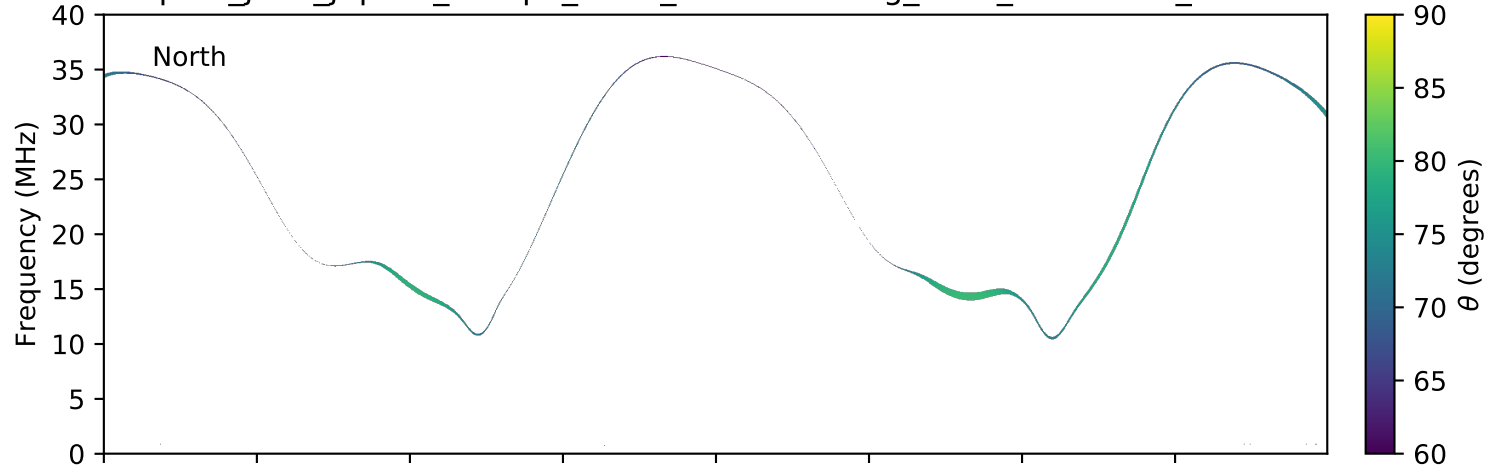
expres_juno_jupiter_europa_isaac_lossc-wid1deg_3kev_20171206_v01.cdf
