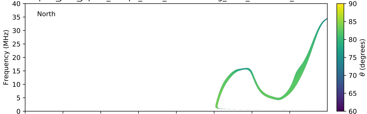
expres_juno_jupiter_europa_isaac_lossc-wid1deg_3kev_20171205_v01.cdf
