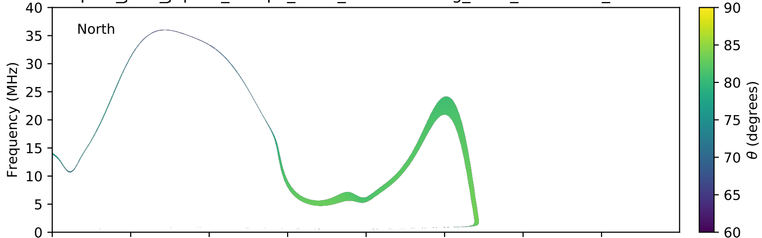
expres_juno_jupiter_europa_isaac_lossc-wid1deg_3kev_20171203_v01.cdf
