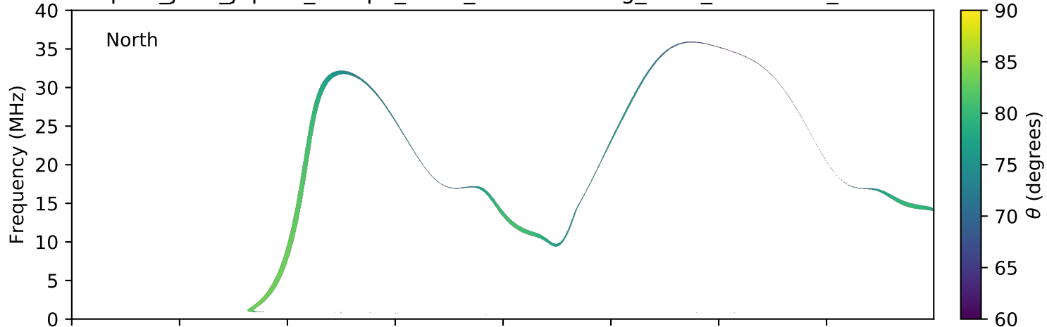
expres_juno_jupiter_europa_isaac_lossc-wid1deg_3kev_20171202_v01.cdf
