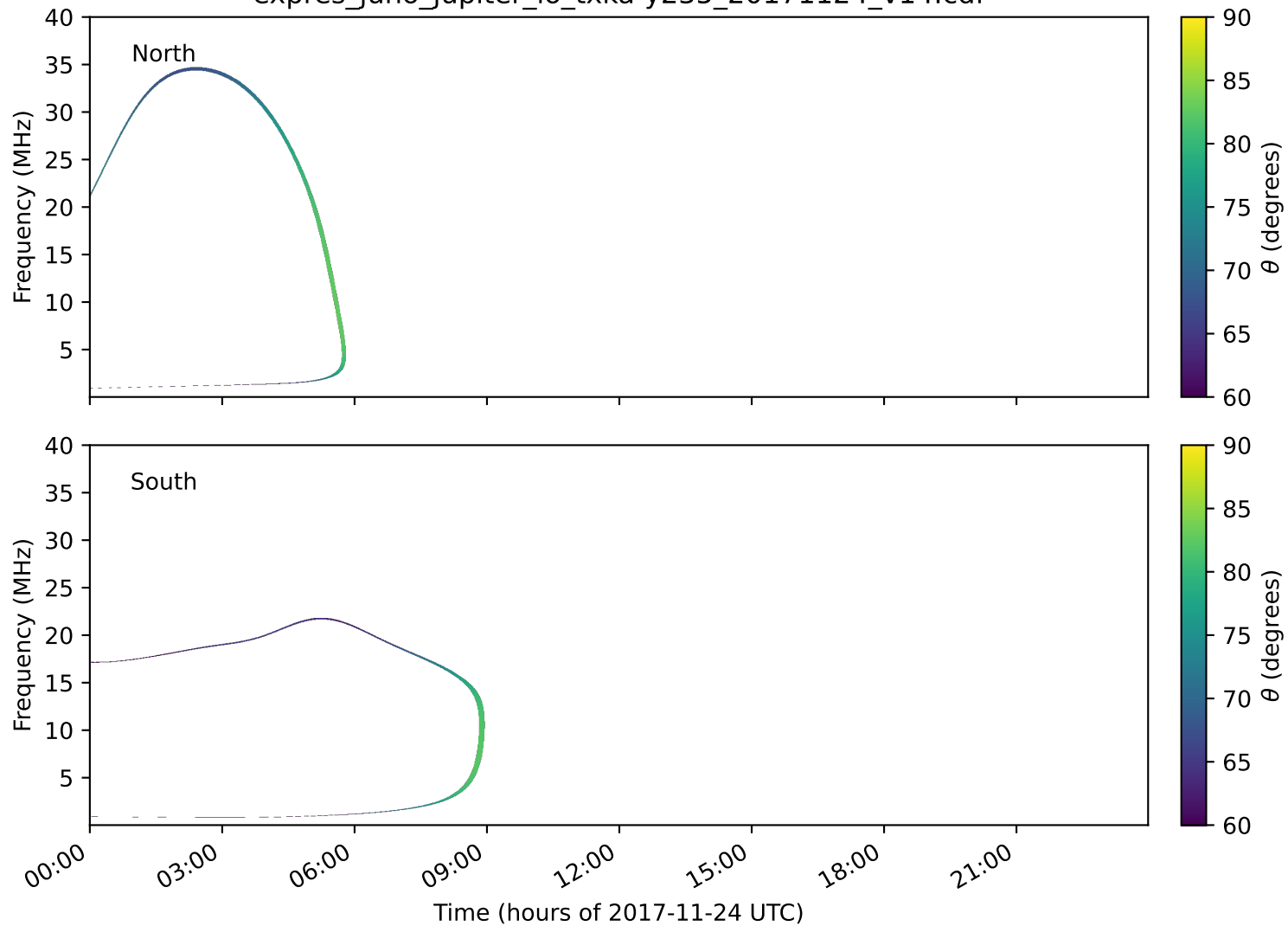
expres_juno_jupiter_io_txka-y235_20171124_v14.cdf
