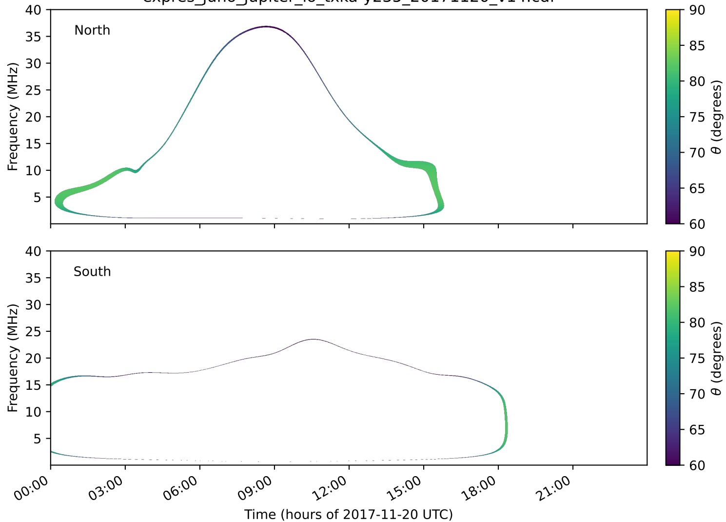
expres_juno_jupiter_io_txka-y235_20171120_v14.cdf
