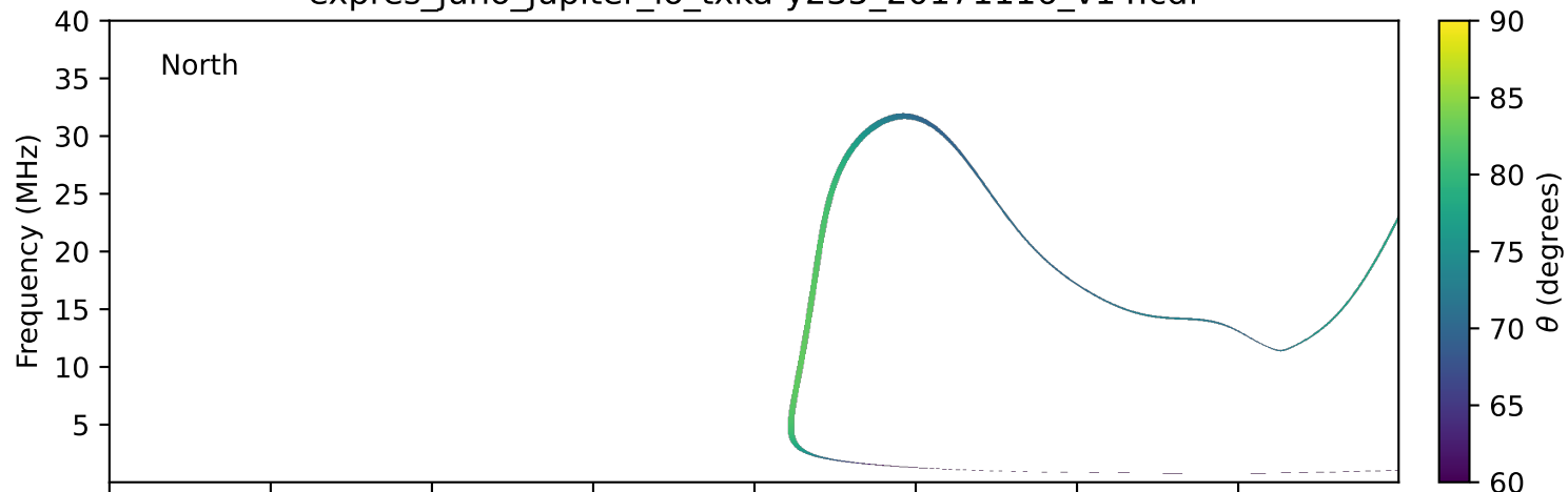
expres_juno_jupiter_io_txka-y235_20171116_v14.cdf
