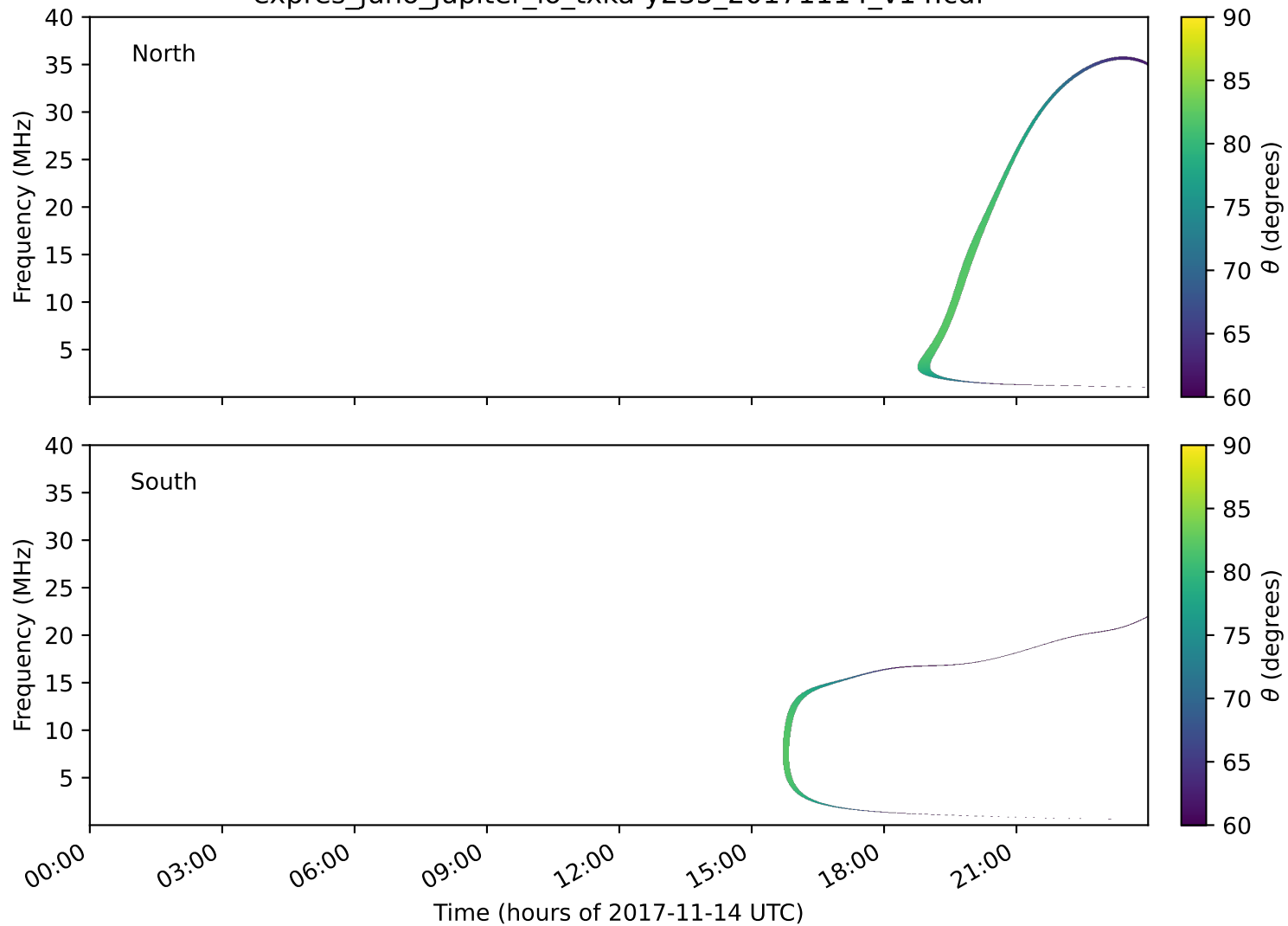
expres_juno_jupiter_io_txka-y235_20171114_v14.cdf
