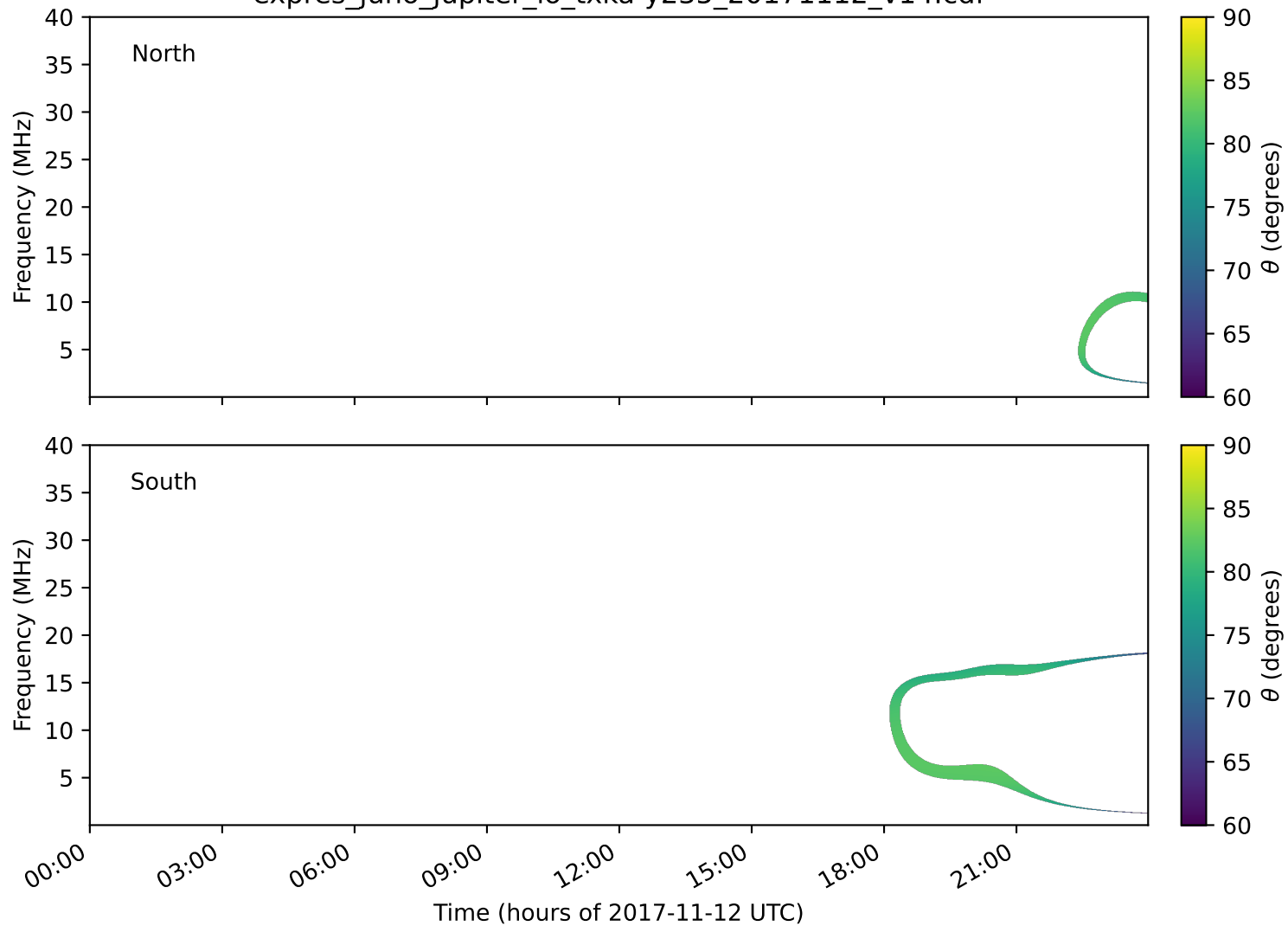
expres_juno_jupiter_io_txka-y235_20171112_v14.cdf
