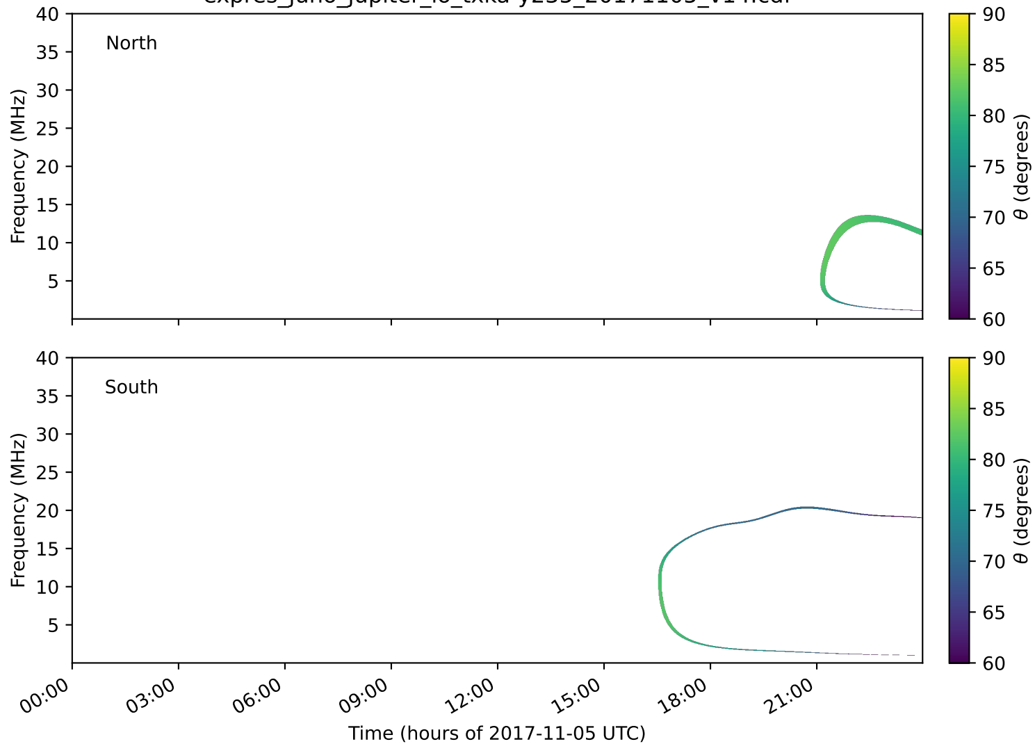
expres_juno_jupiter_io_txka-y235_20171105_v14.cdf
