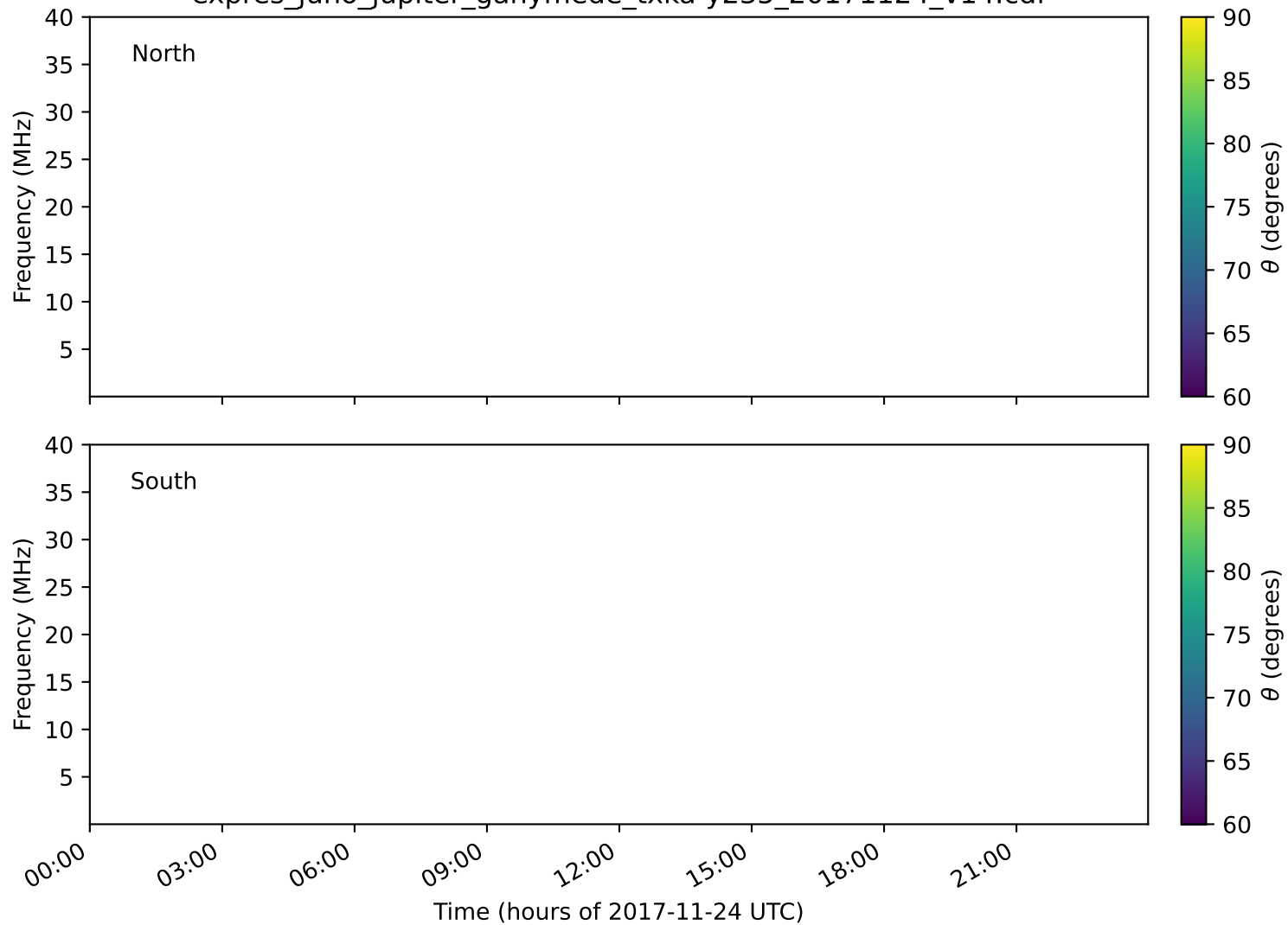
expres_juno_jupiter_ganymede_txka-y235_20171124_v14.cdf
