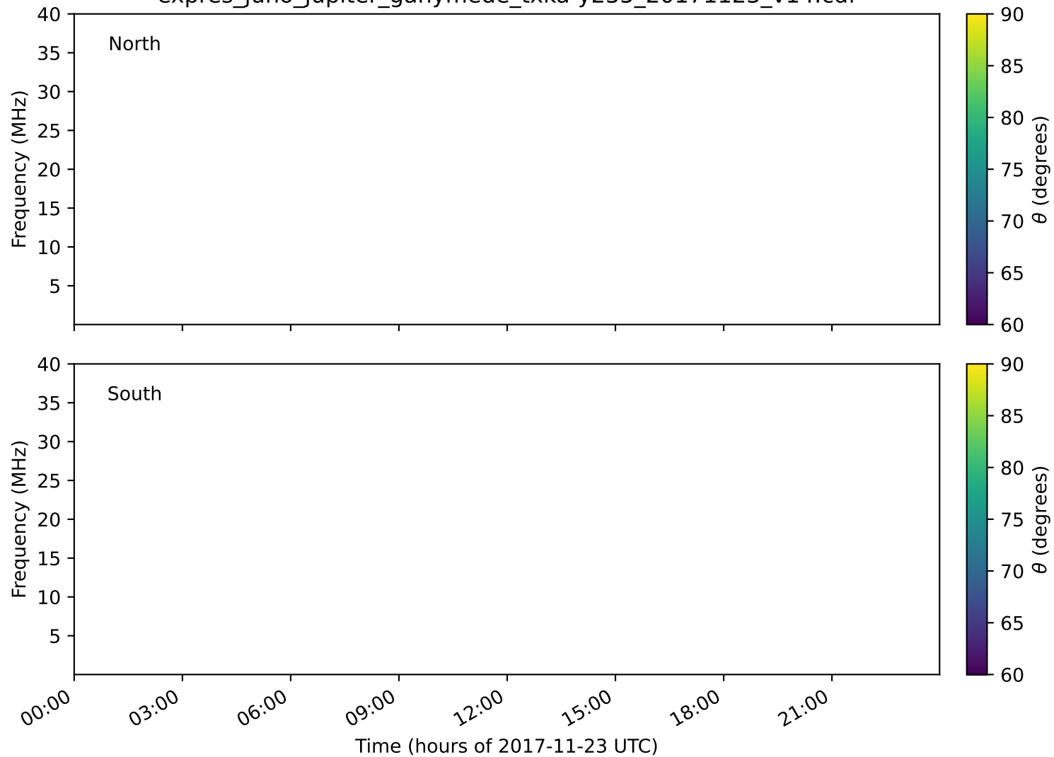
expres_juno_jupiter_ganymede_txka-y235_20171123_v14.cdf
