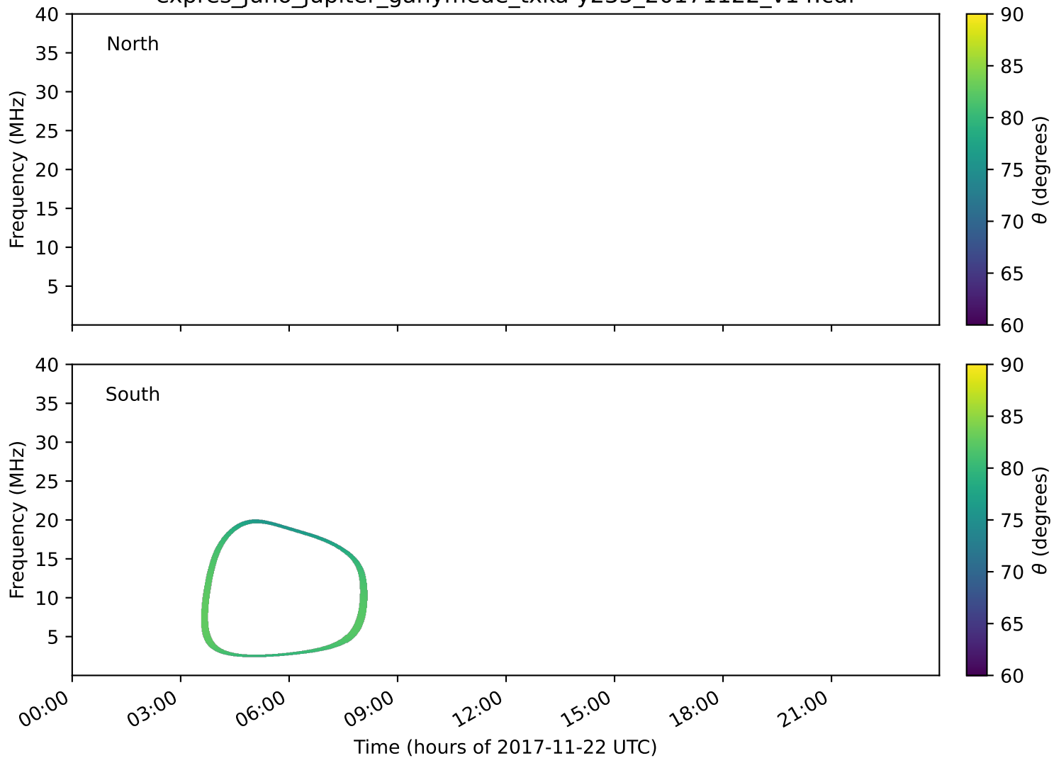
expres_juno_jupiter_ganymede_txka-y235_20171122_v14.cdf
