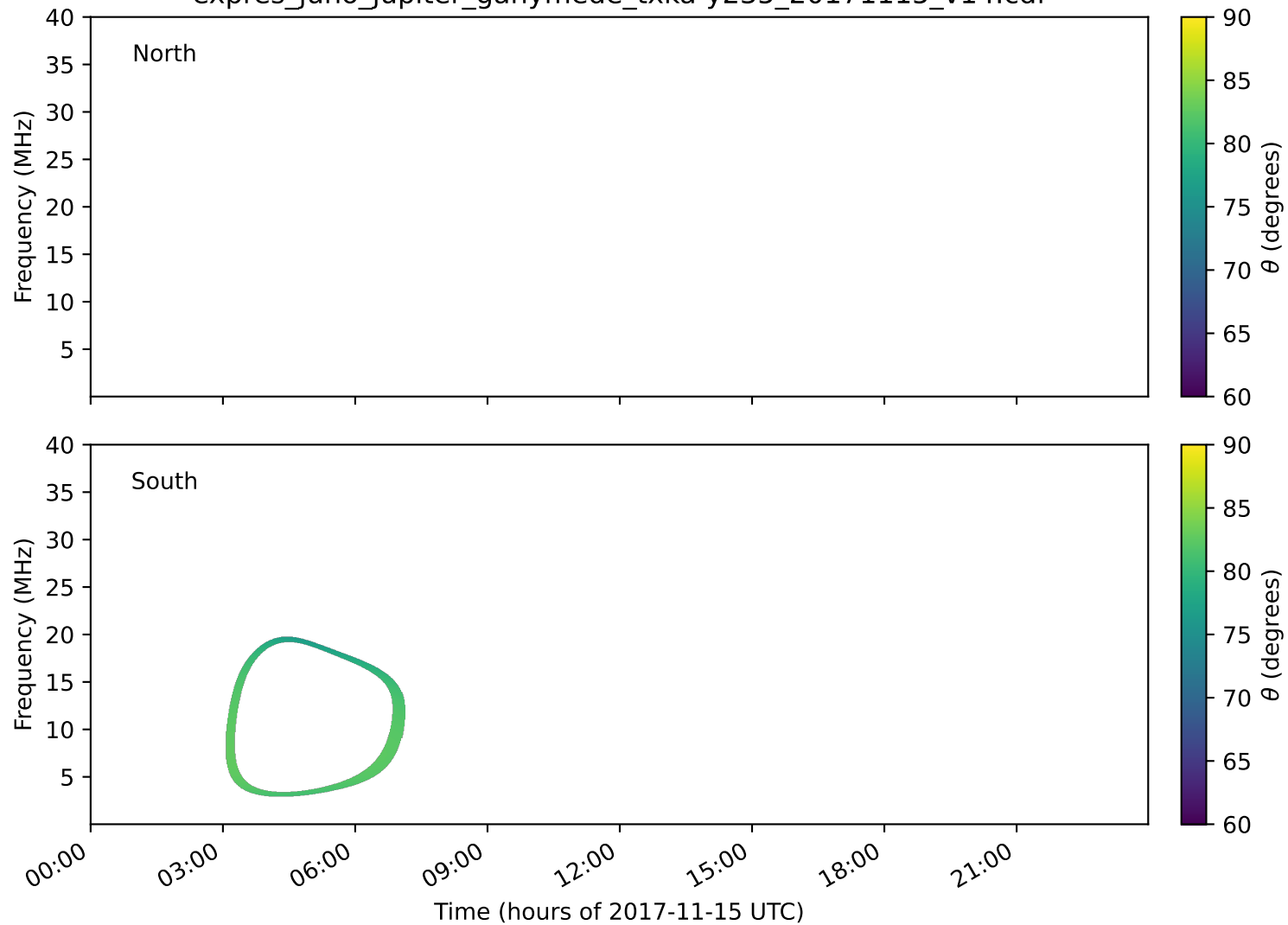
expres_juno_jupiter_ganymede_txka-y235_20171115_v14.cdf
