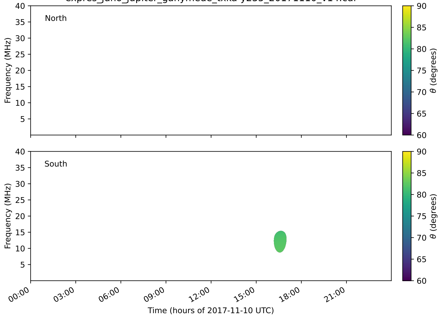
expres_juno_jupiter_ganymede_txka-y235_20171110_v14.cdf
