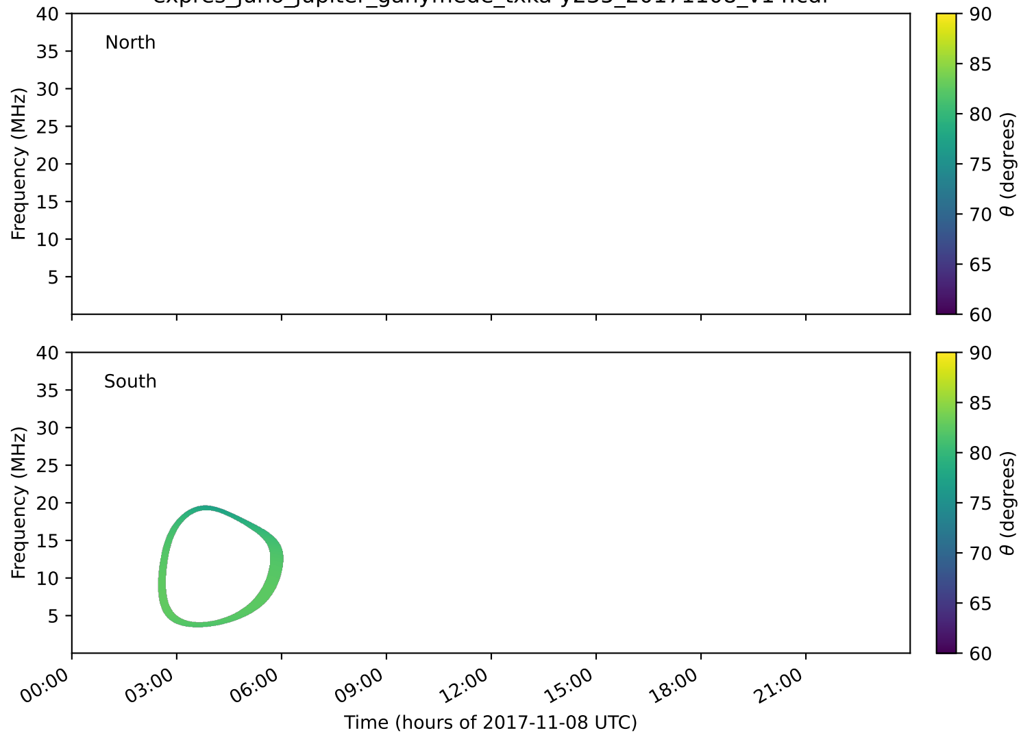
expres_juno_jupiter_ganymede_txka-y235_20171108_v14.cdf
