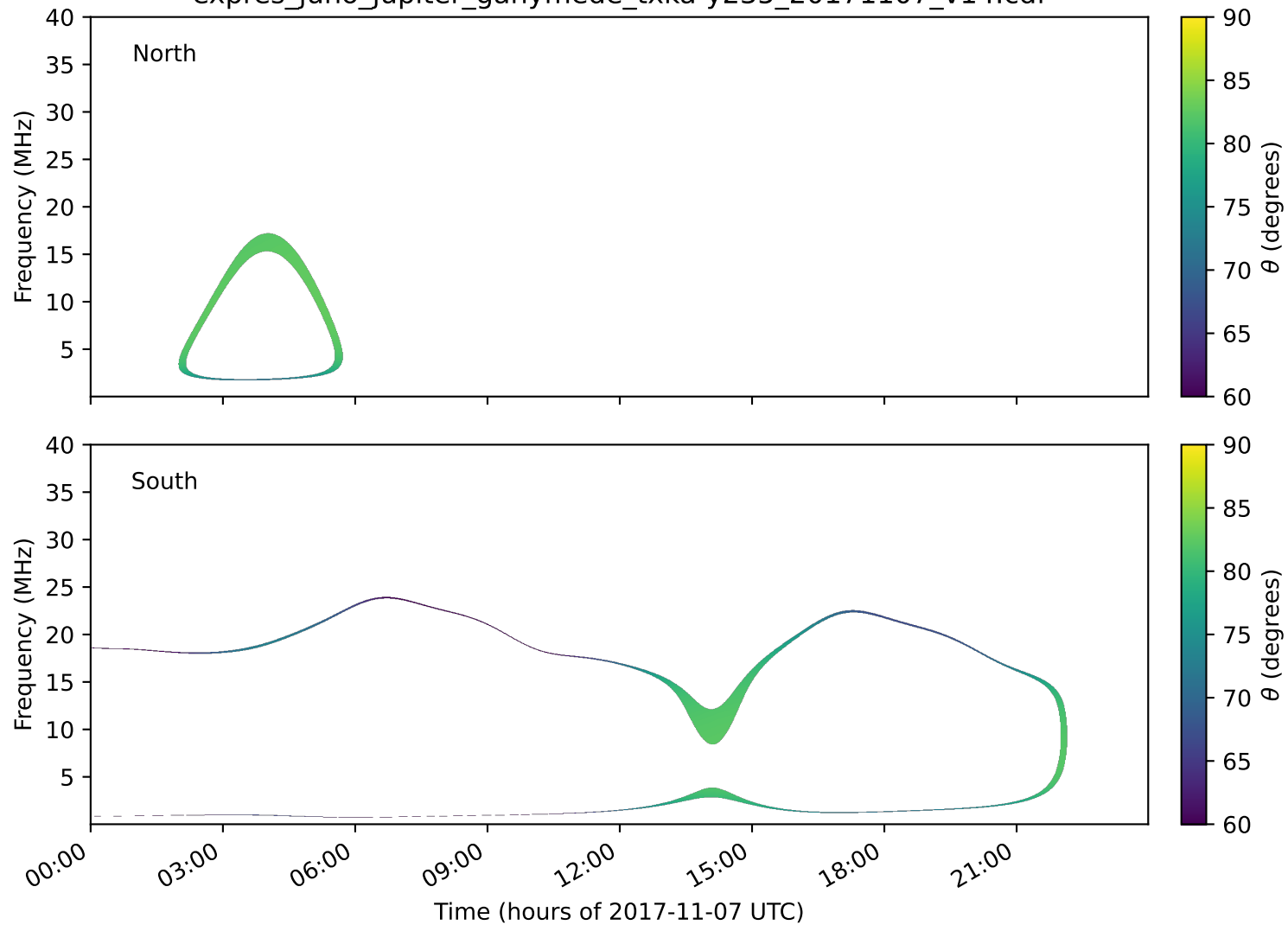
expres_juno_jupiter_ganymede_txka-y235_20171107_v14.cdf
