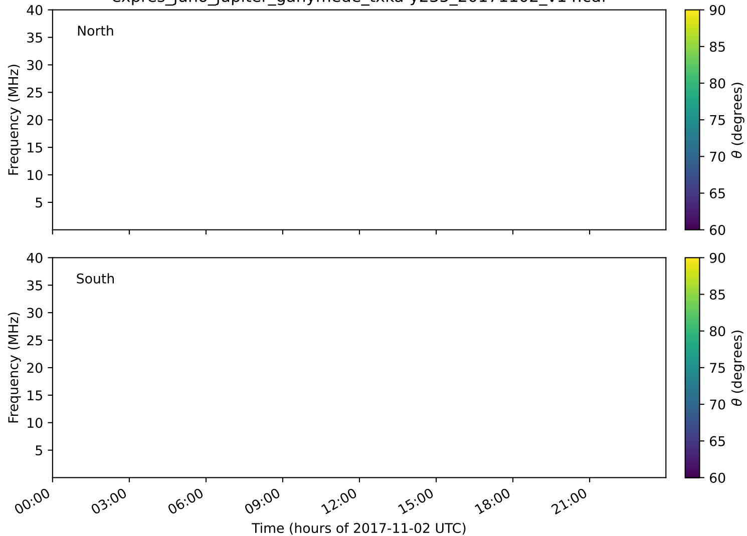
expres_juno_jupiter_ganymede_txka-y235_20171102_v14.cdf
